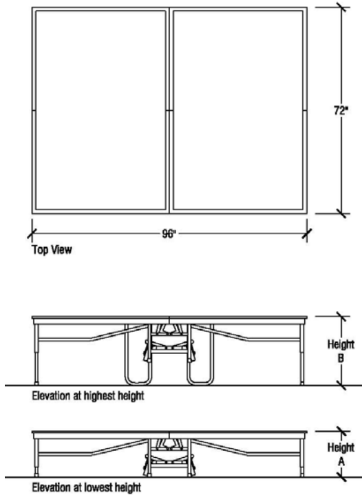
Open Stage Dimensions
