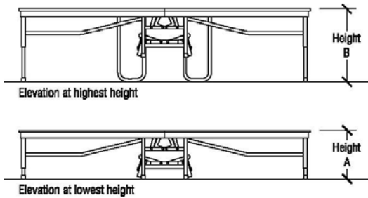
Open Stage Dimensions
