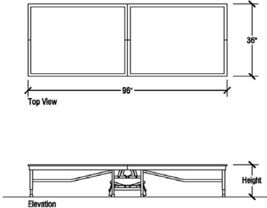
Open Stage Dimensions
